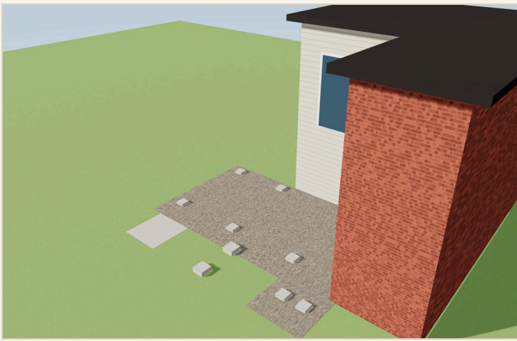
Step 1 · Footings — 9 Diamond Pier DP-50/50 driven-pin footings
