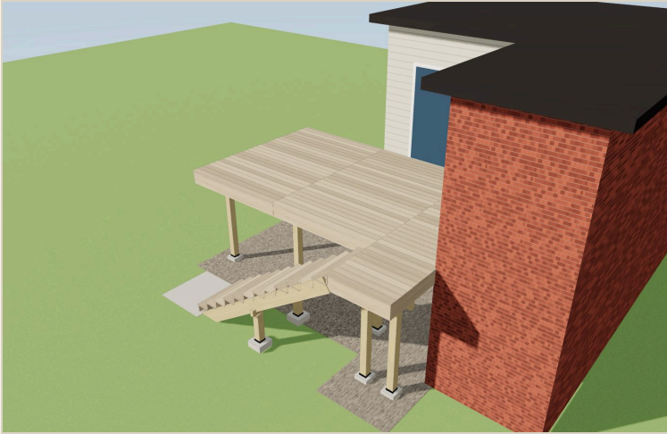
Step 6 · Decking — TimberTech Vintage Weathered Teak, hidden fasteners
