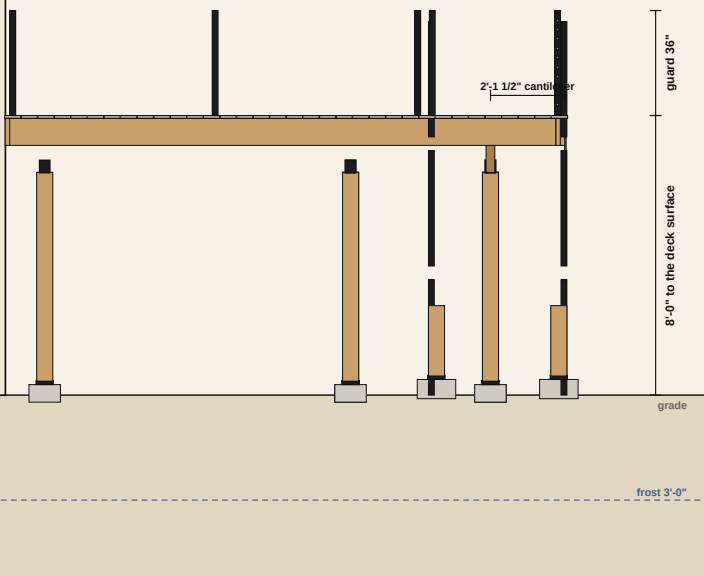
SECTION through zone L at 2'-0" — looking toward the left end
