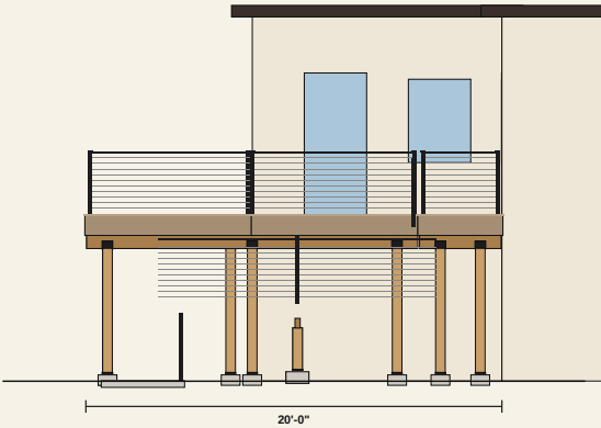
FRONT ELEVATION — from the yard
